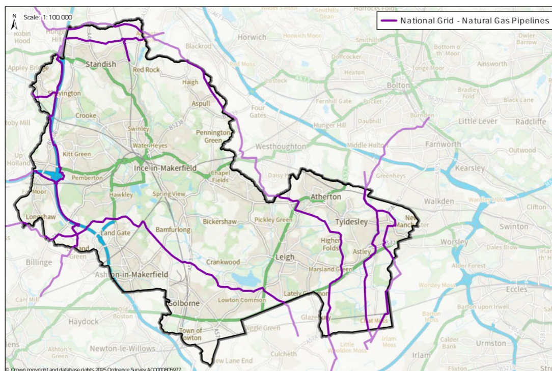
Figure 3.3: Location of National Gas assets in the borough
