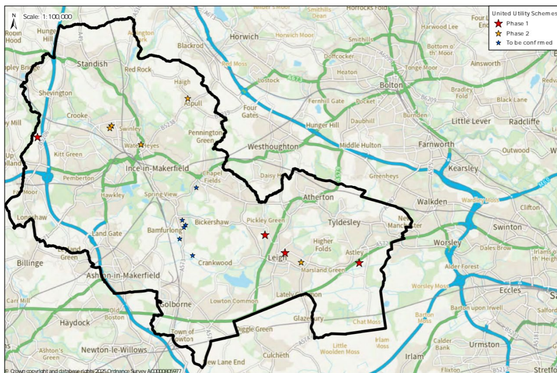
Figure 3.2: Location of planned improvements to combined sewer overflows in the borough
